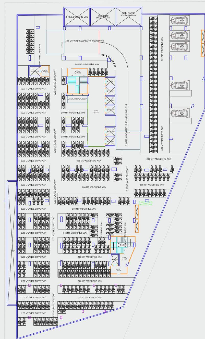
BASEMENT-1 PLAN
